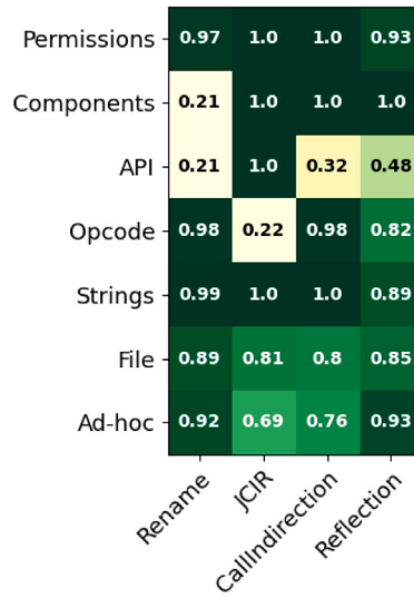
(b) ObfuscAPK vs AAMO
