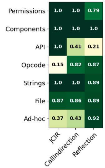
(c) AAMO vs DroidChameleon
