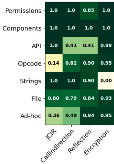
(a) ObfuscAPK vs DroidChameleon
