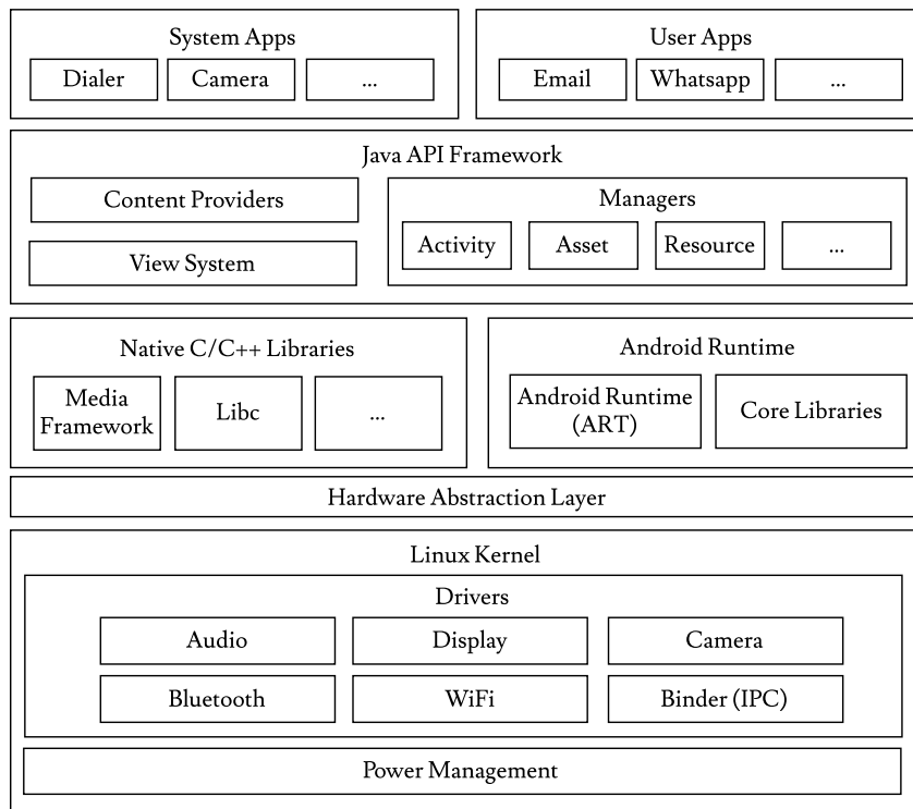
Fig. 1. The Android software stack.
