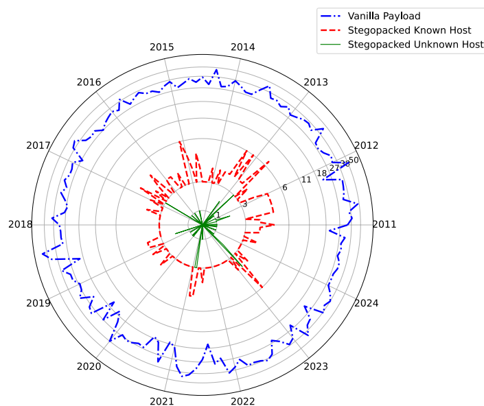
Fig. 12. Total detection comparison (log scale) between unpacked payloads embedded in known and unknown hosts.
