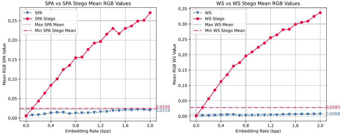
Fig. 18. Steganalysis compares steganographic images and their original version at varying embedding rates.
