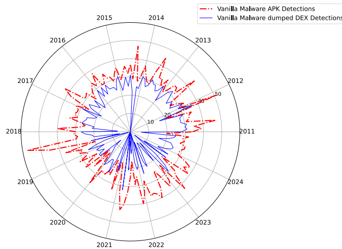
Fig. 19. Detection results: comparison between original malware APKs and their extracted dex files.
