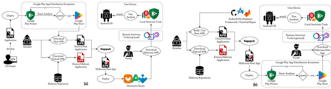
Fig. 3. StegoPack: Threat model using (a) a known app and (b) an unknown app as host.
