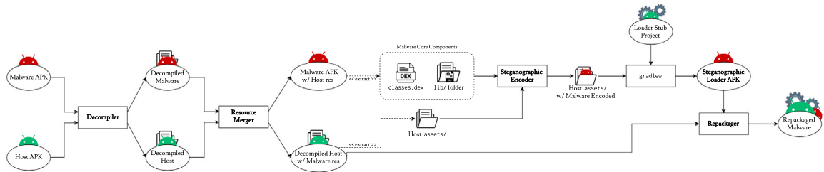
Fig. 4. StegoPack: Malware repackaging workflow.
