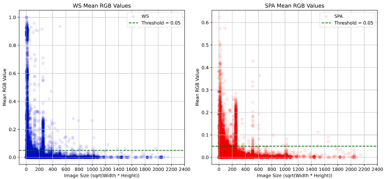
Fig. 24. Steganalysis on goodware assets about image size.
