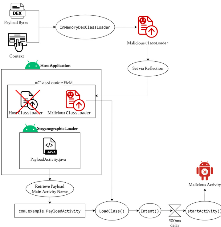
Fig. 8. Substitution of the ClassLoader and Runtime Dispatching of the payload activity from the host.
