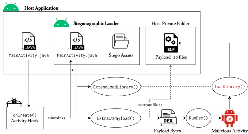
Fig. 7. StegoPack: Payload extraction and loading process.
