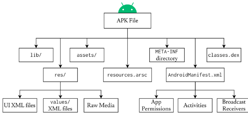
Fig. 2. Structure of a compiled Android APK.
