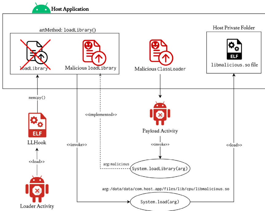
Fig. 9. StegoPack: Dynamic loading of native libraries.
