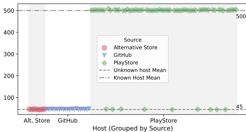
Fig. 11. Scatterplot showing the total number of detections for all stegopacked payloads within each host app, categorized by the host's source.
