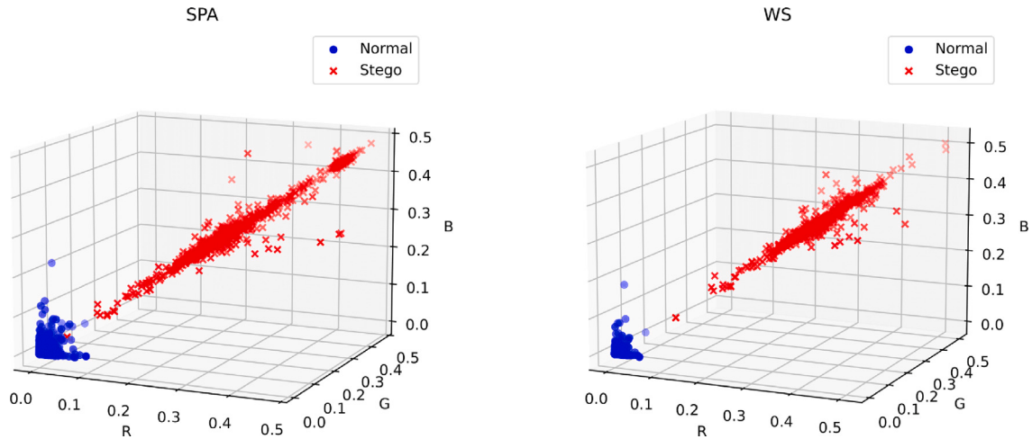
Fig. 17. Distribution of WS and SPA analysis results on R, G, B components.
