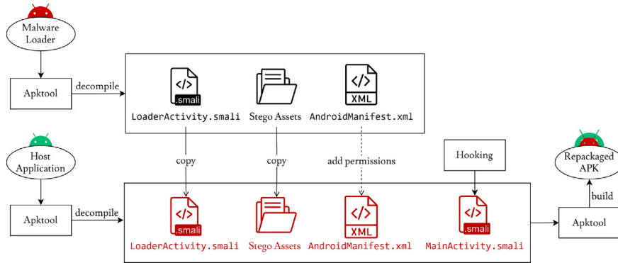
Fig. 6. StegoPack: Workflow of the repackaging process.
