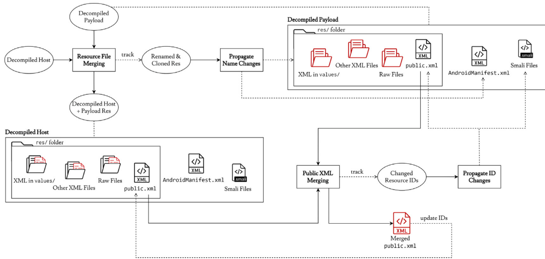
Fig. 5. StegoPack: Resource merger scheme.
